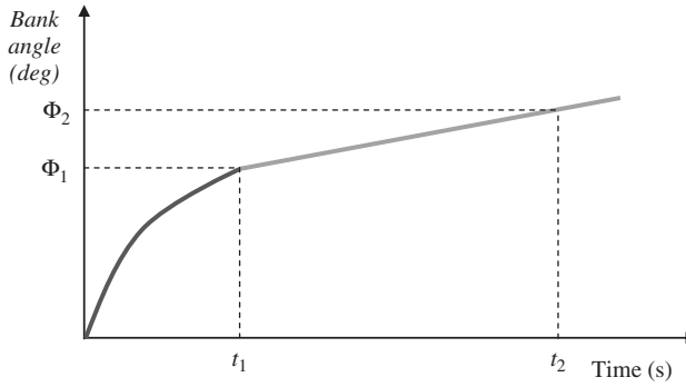
Figure 12.14 Aircraft bank angle response to an aileron deflection
