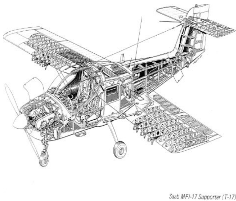
Figure 3.17 Saab MFI-17 supporter. Reproduced from permission of Saab.
