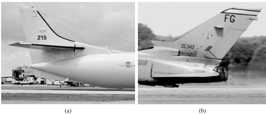
Figure 6.18 An adjustable tail and an all-moving tail: (a) adjustable horizontal tail in Fairchild C-26A Metro III; (b) all-moving tail in Panavia Tornado. Reproduced from permission of (a) Luis David Sanchez; (b) Antony Osborne.
