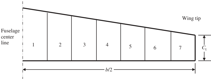
Figure 5.58 Dividing a wing into several sections
