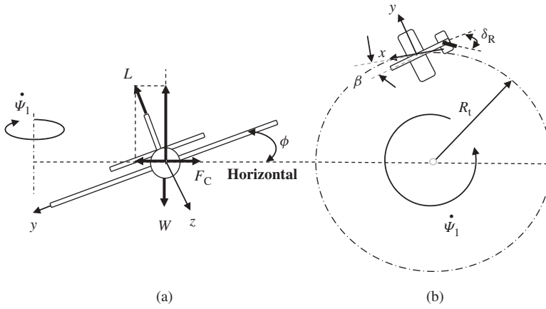
Figure 12.33 An aircraft in a turning flight. (a) Front view; (b) Top view
