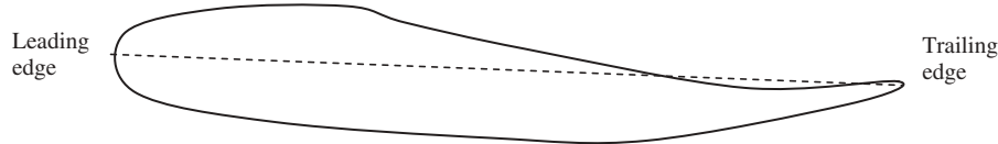
Figure 6.9 A wing airfoil section with reflexed trailing edge
