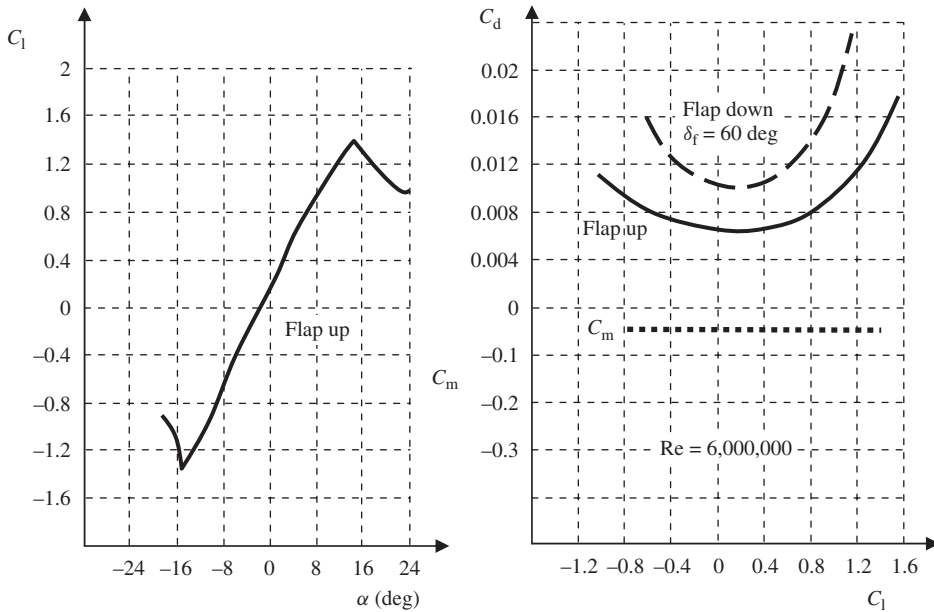
Figure 5.66 Airfoil section NACA 2415. Reproduced from permission of Dover Publications, Inc.
